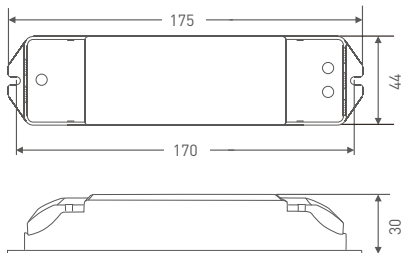
R4-5A/R4-CC Receiver
